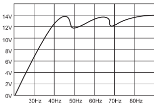
Bassperformance at 50Hz and 70Hz without capacitor
