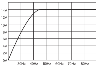
Bassperformance at 50Hz and 70Hz with capacitor
